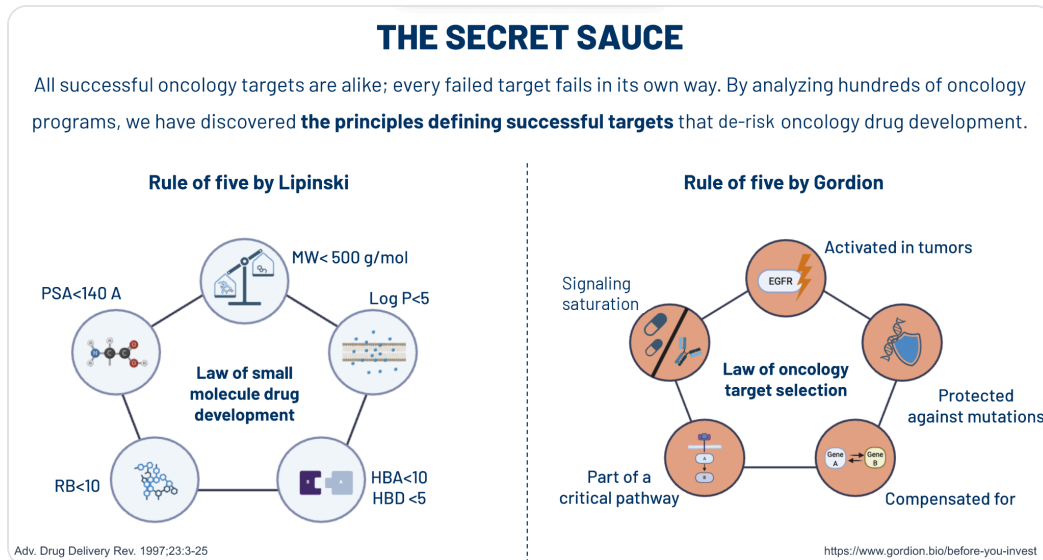
Figure 1. Rule-of-five. Inspired by Lipinski's rule of 5, and the experience of assessing hundreds of oncology drug programs, a handful of simple rules characterising successful drug targets emerged.
